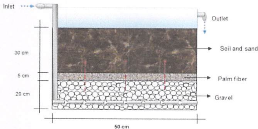
Figure 1 Reactor Constructed Wetland
